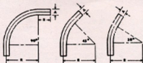
STANDARD RADIUS BEND DIMENSIONS
